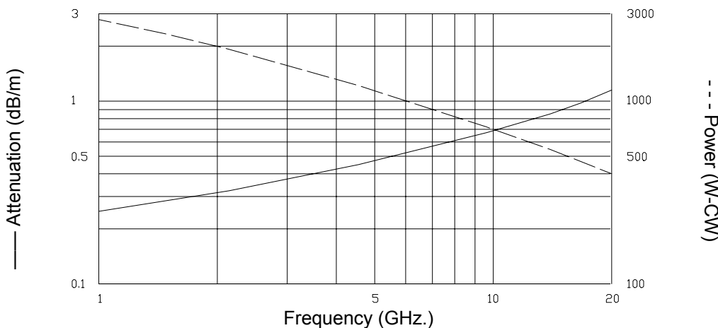
Attenuation Power
