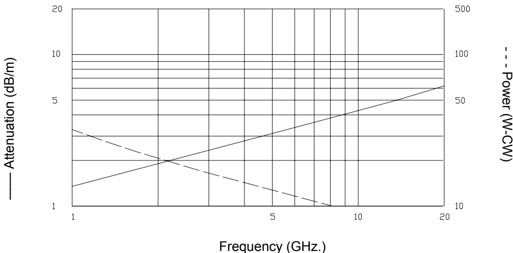
Attenuation Power
