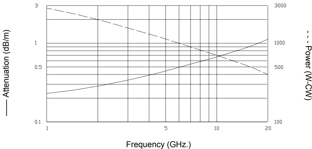
Attenuation Power
