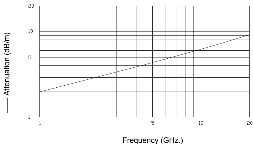
Attenuation Power
