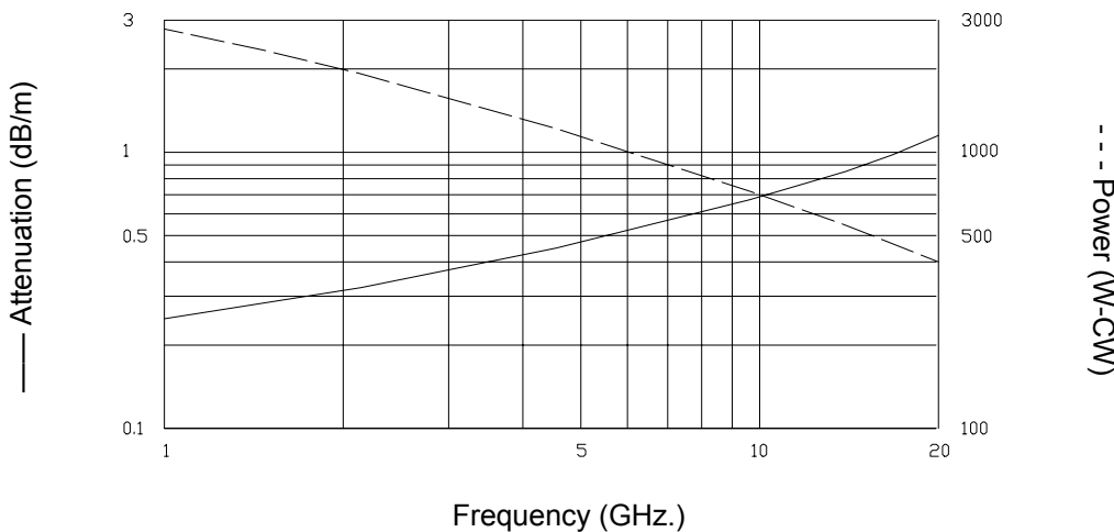
Attenuation Power
