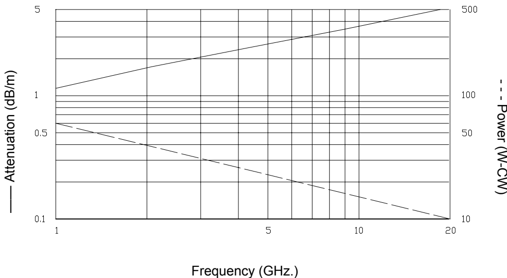
Attenuation Power
