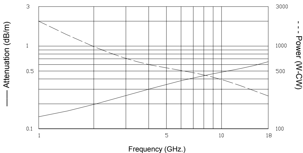
Attenuation Power
