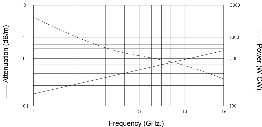
Attenuation Power
