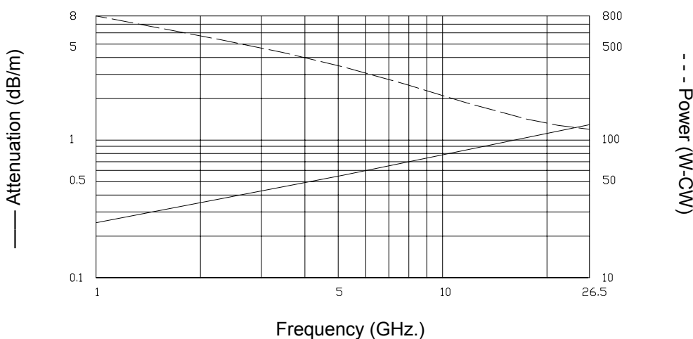
Attenuation Power
