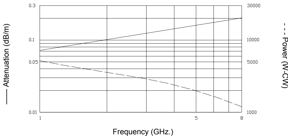
Attenuation Power
